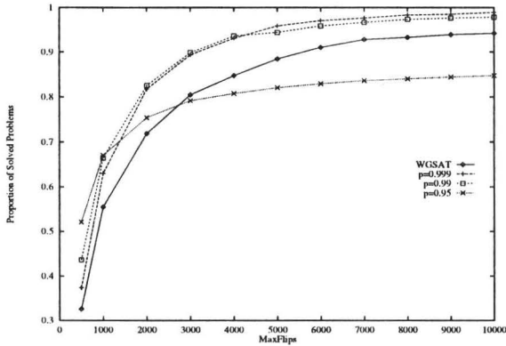
Figure 5: Satisfiability Performance of WGSAT With Varying Decay Rates and Learning Rate of 1.
