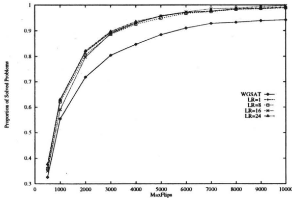
Figure 2: Satisfiability Performance of WGSAT With Varying Learning Rates and Decay Rate of 0.999.
