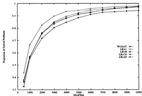
Figure 3: Satisfiability Performance of WGSAT With Varying Learning Rates and Decay Rate of 0.99.
