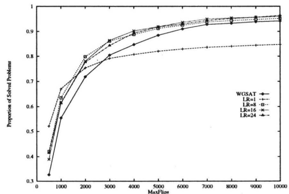
Figure 4: Satisfiability Performance of WGSAT With Varying Learning Rates and Decay Rate of 0.95.
