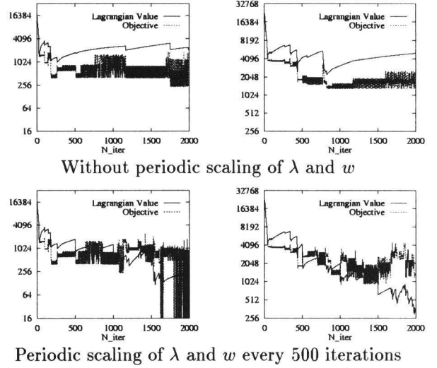
Figure 2: Execution profiles of jnh1 (left) and jnh10 (right). jnh1 is satisfiable and jnh10 is not.
