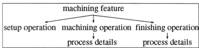
Figure 9: Task decomposition in IMACS.
