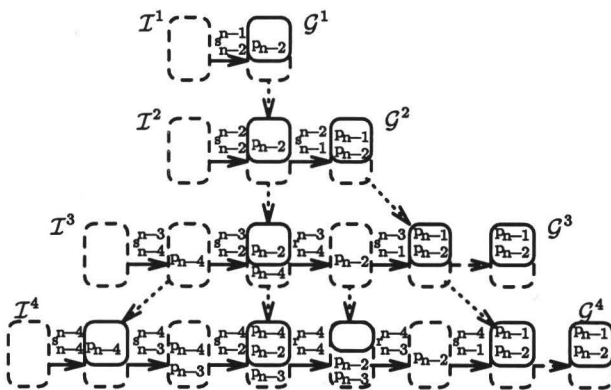
Figure 3: Applying HPLAN to \Sigma_n under \mathcal{H}_2 .
