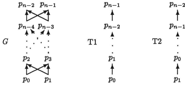
Figure 5: The preorder on \mathcal{P} induced by the first step of the ALPINE algorithm and two of the possible topological sortings of the reduced graph.
