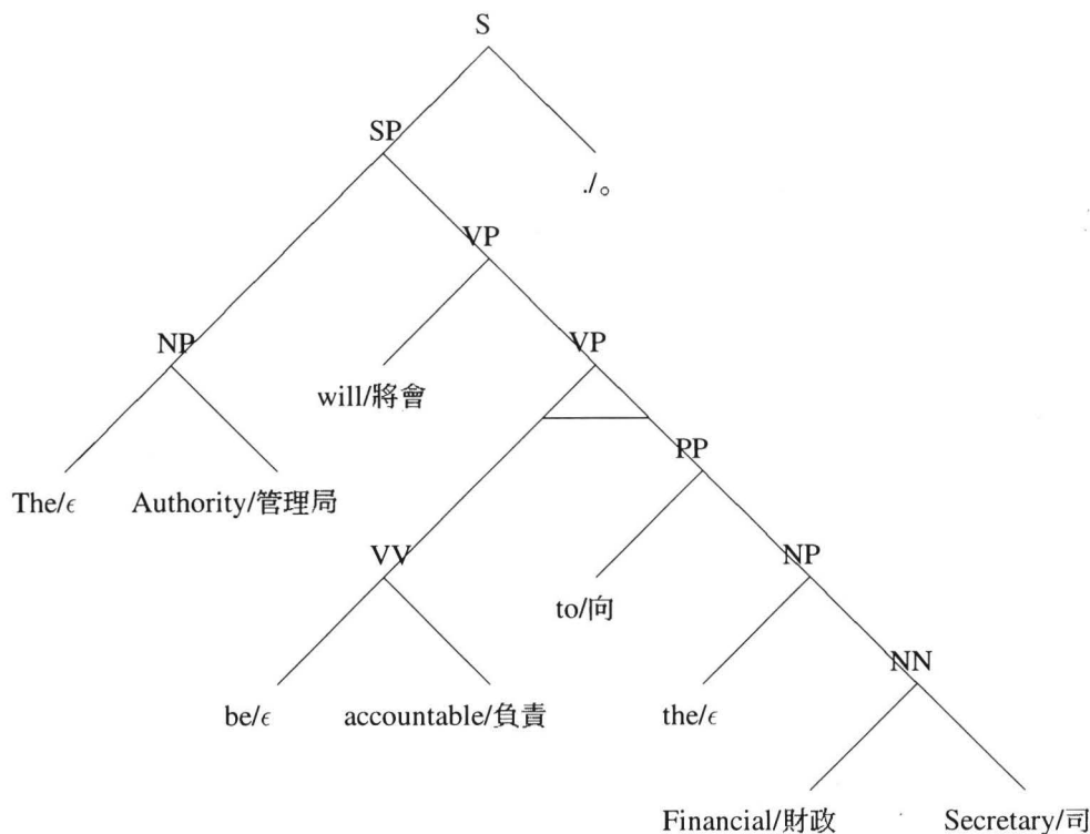
Figure 2: Inversion transduction parse tree.
