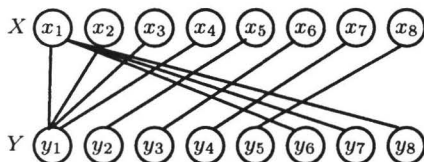
Figure 4: Analysis.
