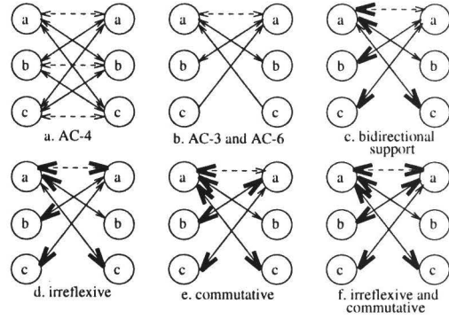
Figure 1: Making inferences.
