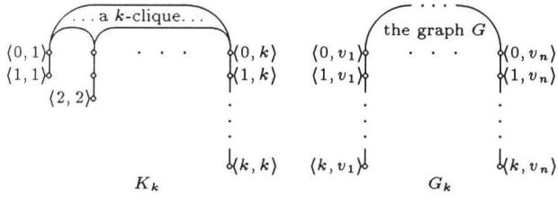
Figure 1: the graphs K_k and G_k
