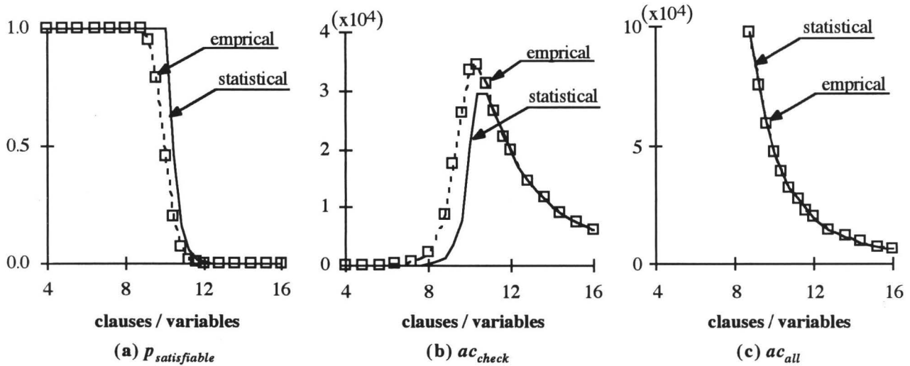
Figure 4: 4-SAT with 50 variables
