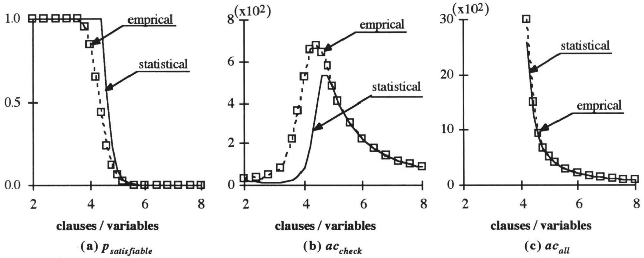
Figure 3: 3-SAT with 50 variables
