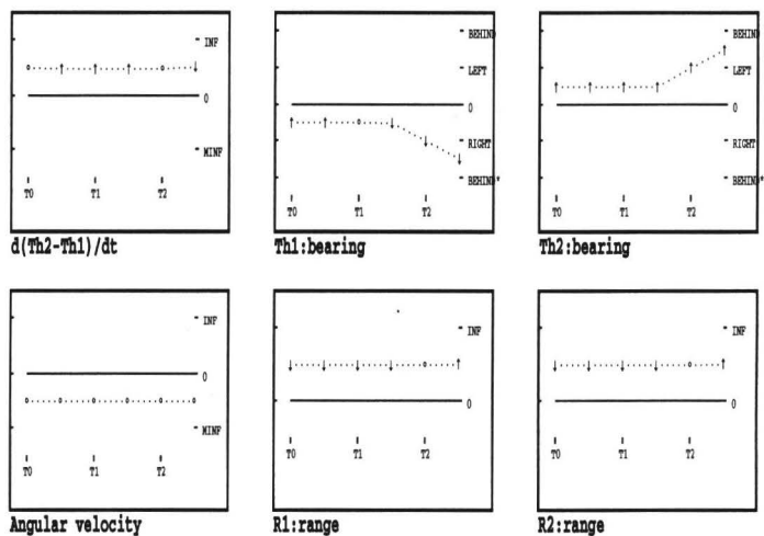
Figure 6: QSim generated behaviours
