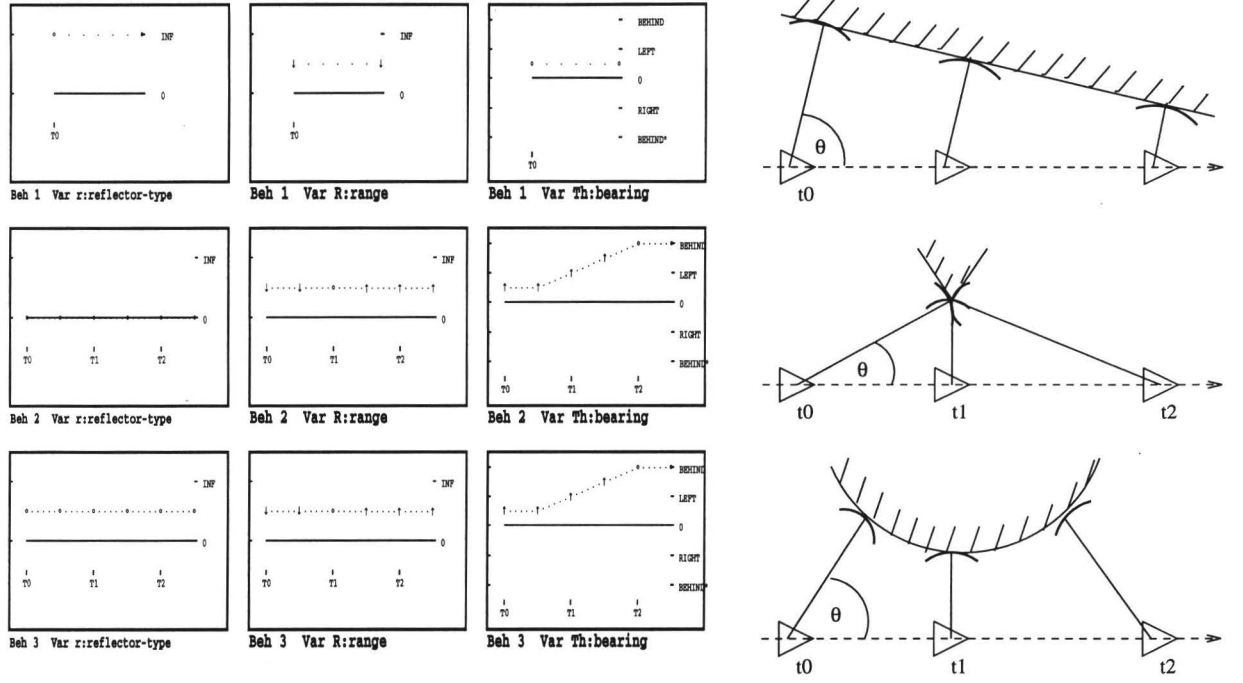
Figure 4: QSim generated behaviours
