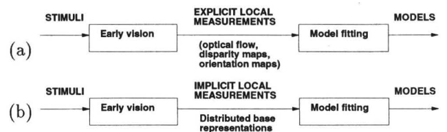
Figure 3: Architectures. (a) Standard computer vision approaches to fit models to explicit representations of local structure, which is prone to failure where explicit representations of local structure cannot be accurately recovered. (b) We advocate fitting models to distributed representations of local structure.
