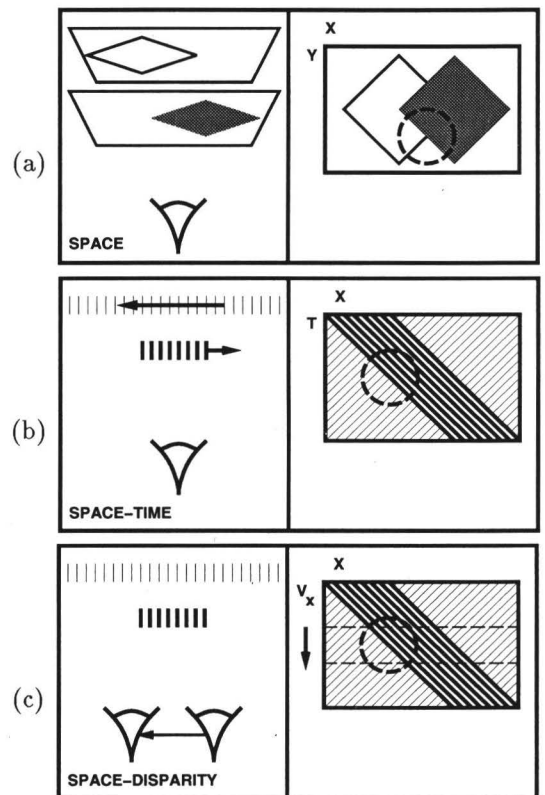
Figure 1: Orientation analysis in three modalities. (a) Edges and texture are oriented in space (x, y) ; (b) Motion is orientation in space-time (x, t) ; (c) Stereo is orientation in space-disparity (x, V_x) .
