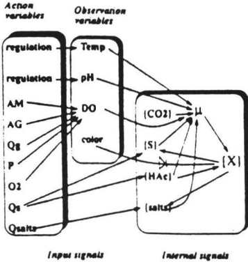
Fig.3 Causal network of a fed-batch fermentation process.
