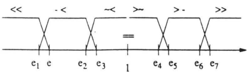
Fig.1: Fuzzy extension to order of magnitude formalism. e < 0.4656 ; e_1 = e/(1+e) ; e_2 = (1+e)^{-2} ; e_3 = (1+e)^{-1} ; e_4 = 1/e_3 ; e_5 = 1/e_2 ; e_6 = 1/e ; e_7 = 1/e_1 .
