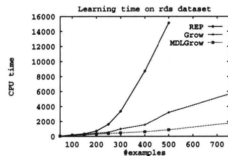
Figure 3: CPU time comparison on rds dataset
