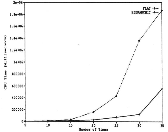
Figure 7: Multiprocessor Scheduling Problem Results: Hierarchic (Solid) v. Flat (Dotted)
