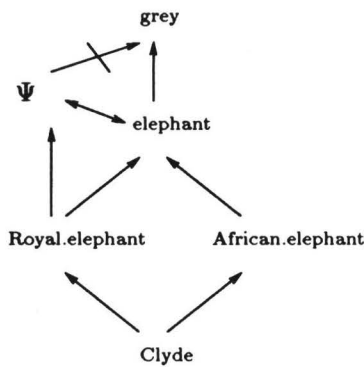
Figure 7: The EIL representation of the Clyde — African.elephant structure
