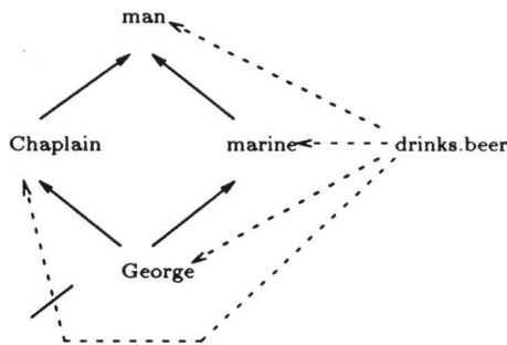
Figure 8: The George example represented in EIL
