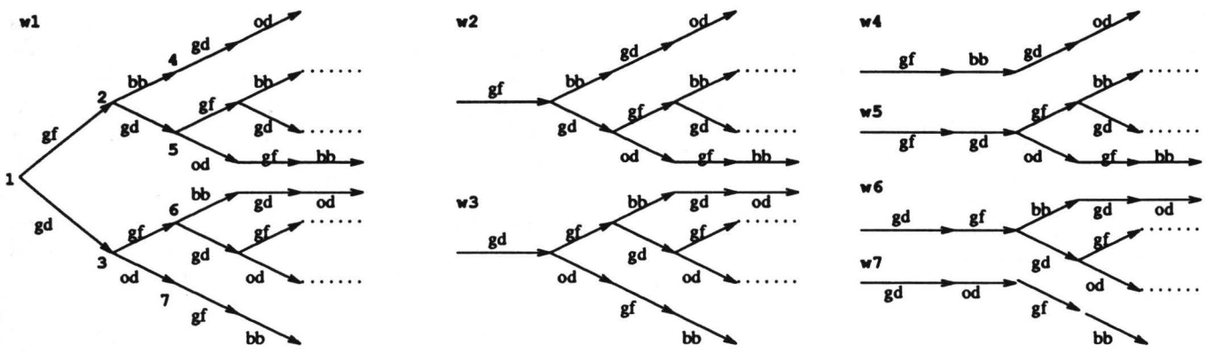
Figure 1: A partial structure of M_1
