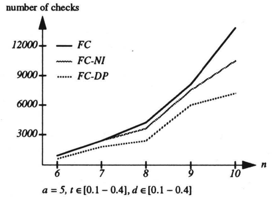
Figure 3: The effects of the use of interchangeability w.r.t. the number of variables.
