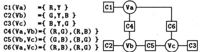
Figure 1: Constraint Network A: Variables are represented by circles and constraints by rectangles. An edge between a circle and a rectangle means that the corresponding variable belongs to the constraint represented by the rectangle.
