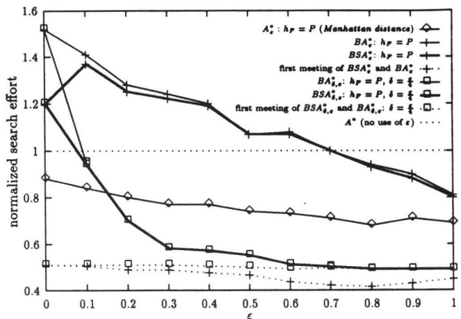
Figure 4: Comparison on the 8-Puzzle (500 instances).
