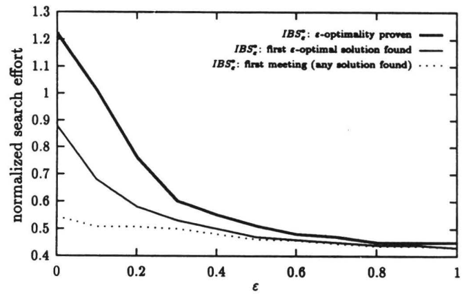
Figure 1: Phases of IBS_\epsilon^* (on the 8-Puzzle).
