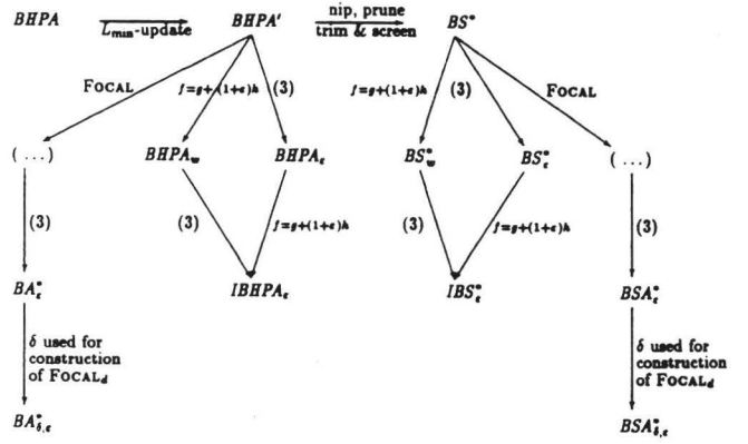
Figure 2: Overview of \epsilon -admissible bidirectional search algorithms.
