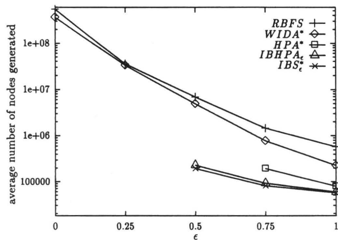
Figure 3: Comparison on the 15-Puzzle (100 instances).
