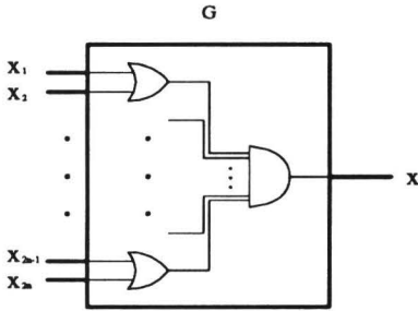
Figure 1: A “black-box” circuit
