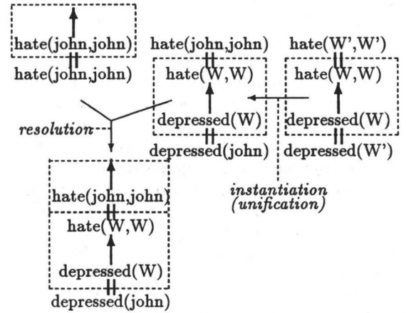
Figure 3: an inference with explanation structures.
