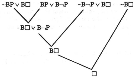
Figure 1. A derivation of \square from the belief-clauses \{\neg BP \vee B\square, BP \vee B\neg P, \neg B\neg P \vee B\square, \neg B\square\} .
