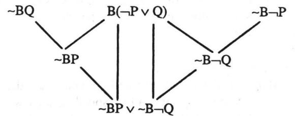
Figure 3. An example where \square cannot be derived.
