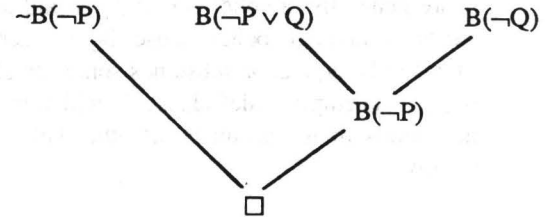
Figure 2. An illustration of resolution proof for beliefs.
