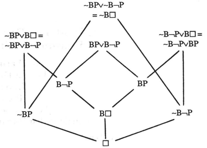
The subsumption relationships among the belief-clauses in a single proposition P .
