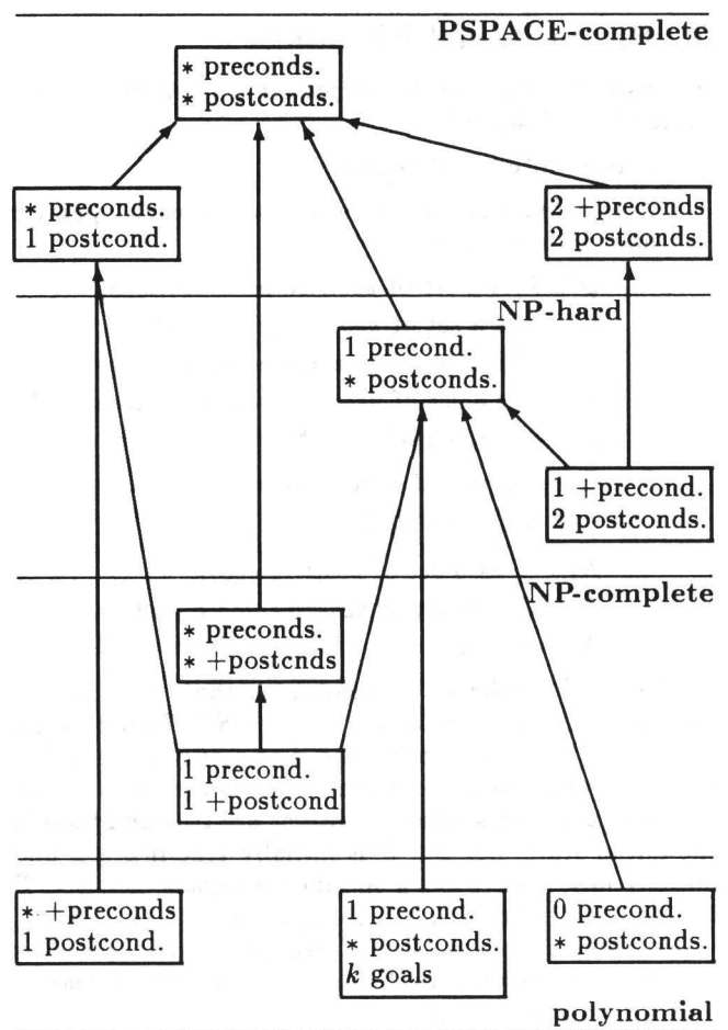
Figure 1: Complexity Results for Hierarchy of Propositional Planning Problems
