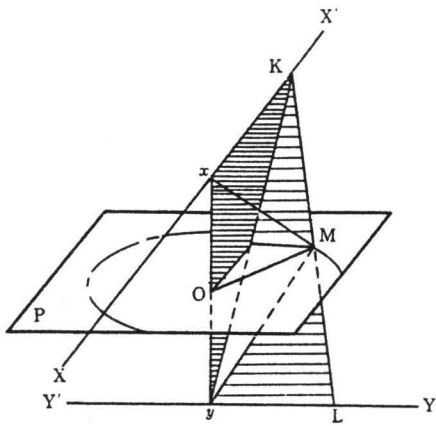
Fig.6 Skew-line problem
