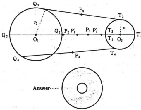
Fig.5 Two-circle problem
