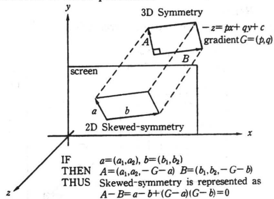
Fig.1 Skewed symmetry
