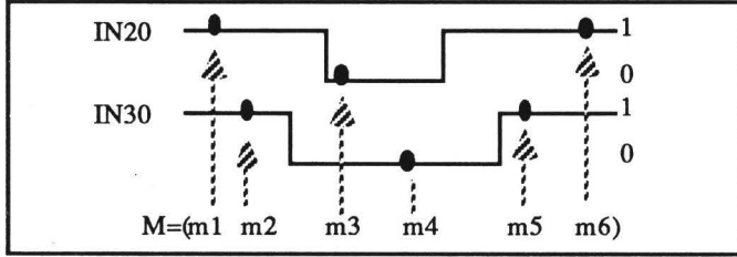
Fig. 3 – M is compatible with other situations
