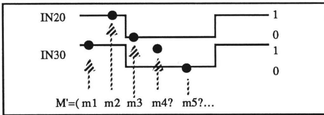
Fig. 5 – Detecting an overlap that should not be there
