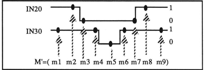
Fig. 4 – A matching measurement sequence
