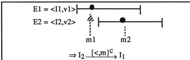
Fig. 6 - The observation rule
