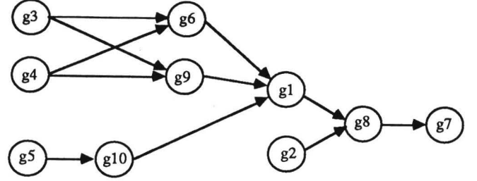
Figure 2: Subgoal Ordering Constraints
