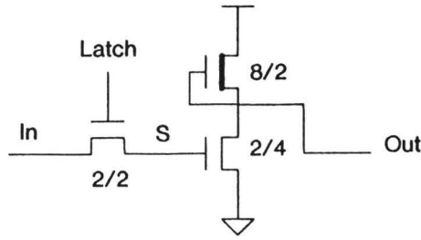
Figure 1: A Inverting Latch.
