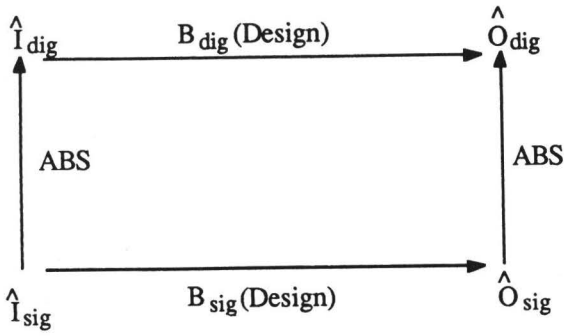
Figure 2: The relationship between B_{sig}(Design) and B_{dig}(Design) . Given ABS and B_{sig}(Design) , B_{dig}(Design) is projected from B_{sig}(Design) according to this diagram. The commutativity need only hold when ABS(i) and ABS(B_{sig}(Design)(i)) are valid.
