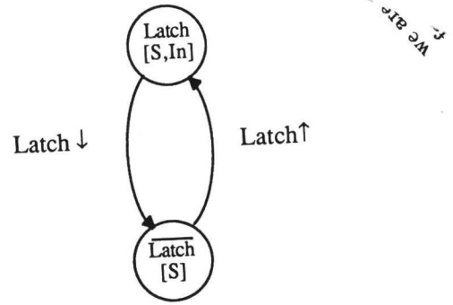
Figure 3: The net transition graph of the Inverting Latch's S node. The S node can be member of two nets, one consisting of just the S node, written [S] , and one consisting of the In and S nodes, written [S, In] .
