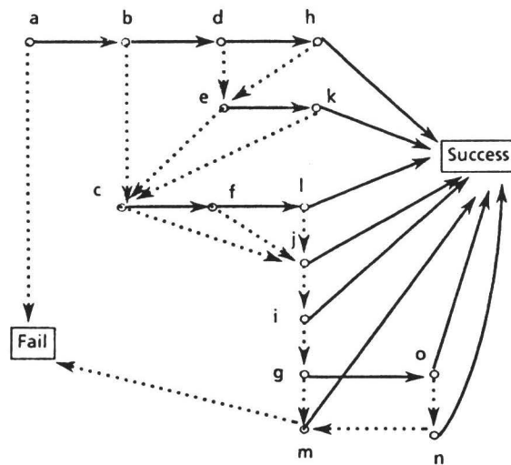
Figure 3: The threaded decision graph for the search space in figure 1. In this figure, solid lines represent success threads, while the dotted ones the failure ones.
