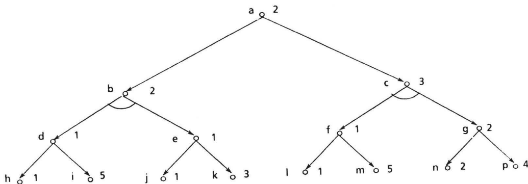
Figure 4: An example AND/OR tree in the worst case situation.
