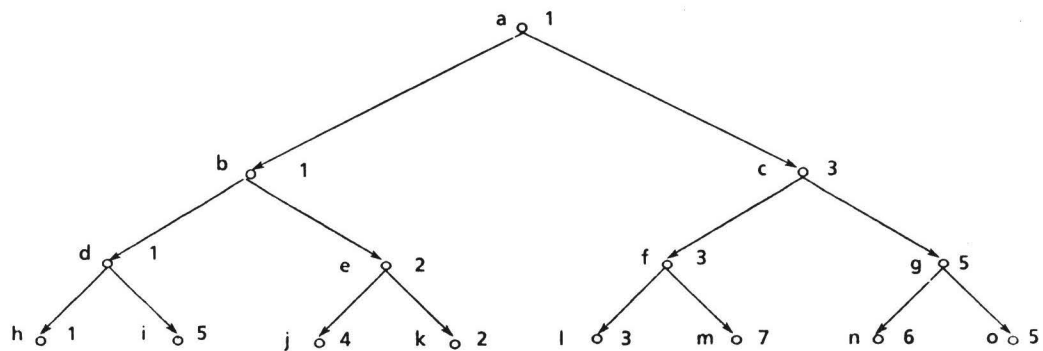
Figure 1: An example search space. The numbers associated with the nodes are their cost values.
