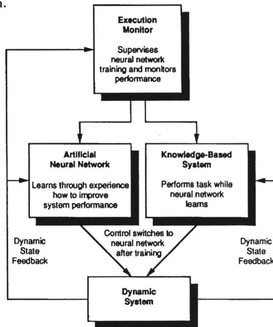
Figure 1. Integration of Neural Network and Knowledge-Based System Techniques for Hierarchical and Modular Control of Dynamic Systems and Learning
