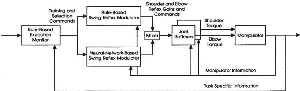
Figure 3. Block Diagram of Manipulator Control System
