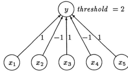
Figure 2 y = x_1 \bar{x}_2 x_3 \bar{x}_4 x_5 .
