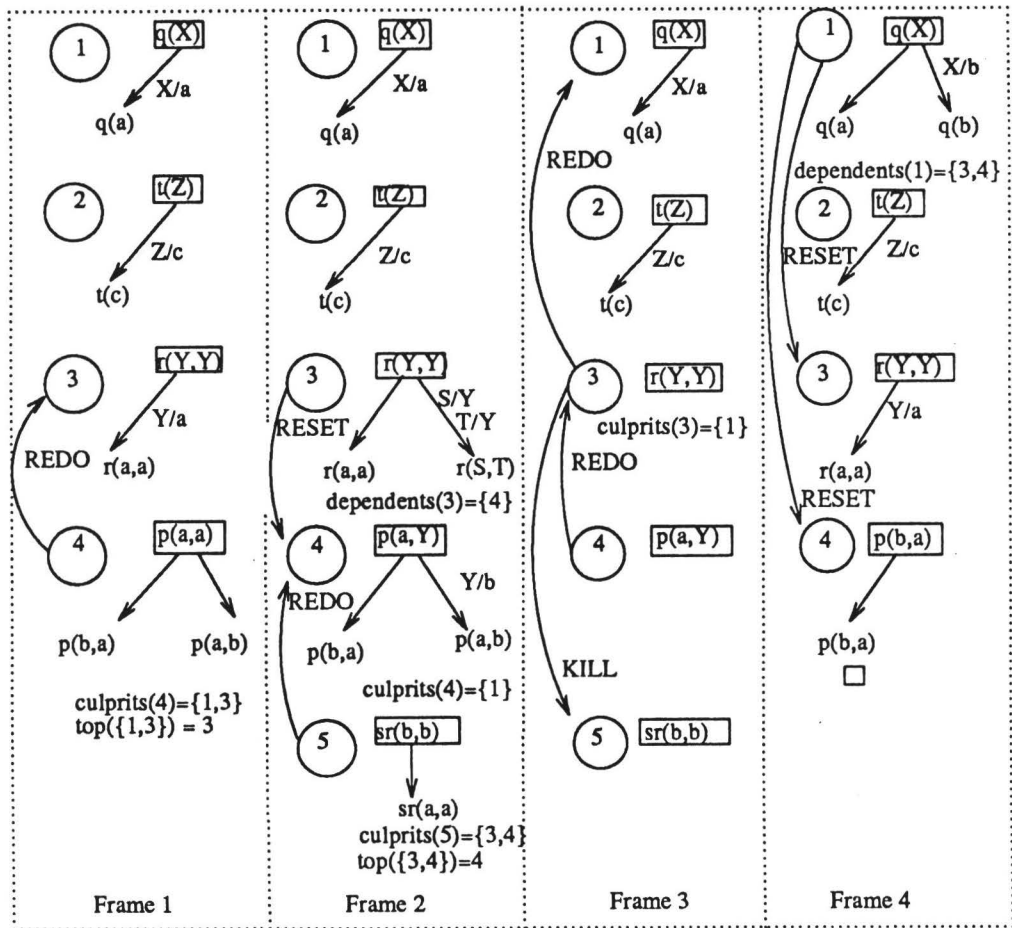
Figure 1. And-parallel execution of a logic program
