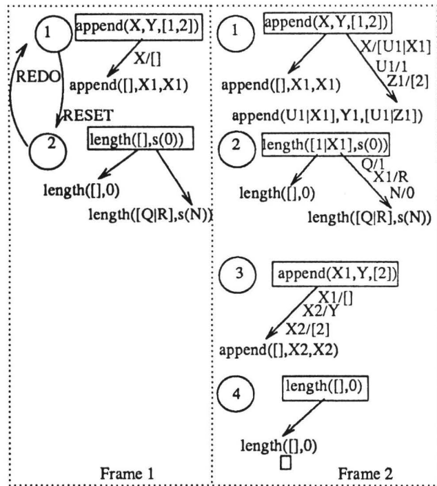
Figure 3. And-parallel execution with stream parallelism
