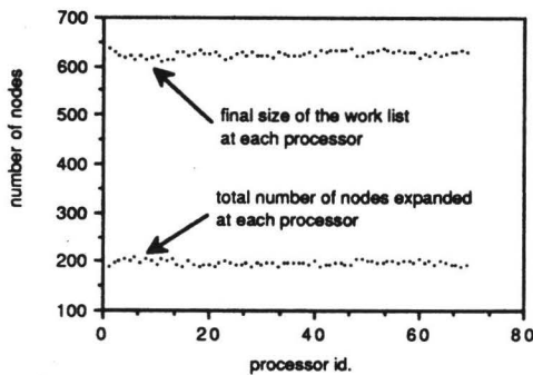
Figure 2: Load Distribution in 70 Processors
