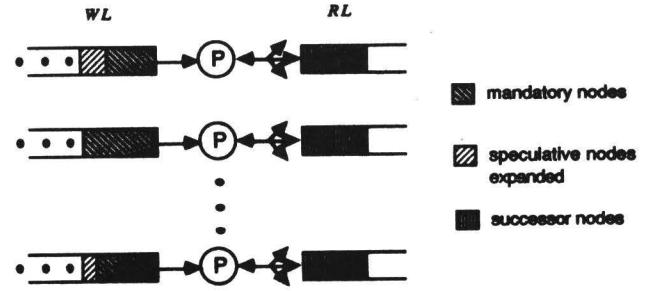
Figure 1: Data Structures and Data Flow in PIA^*
