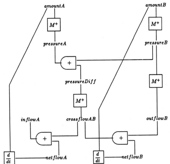
Figure B: Coupled Tank structure
