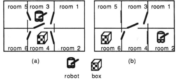
Figure 3. A Robot Planning Example (a). An initial state (2). A goal state
