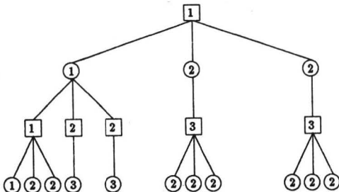
Figure 1: Node types in an optimally ordered tree
