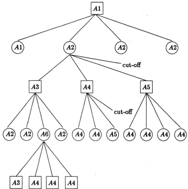
Figure 4: An averagely ordered \alpha\beta -tree ( w = 4, g = 2 )
