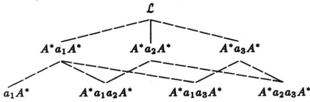
Figure 1: A plan specialization lattice.
