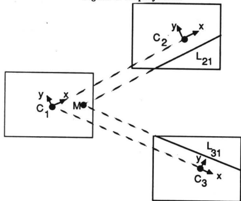
Figure 3: Choice of the coordinate systems on the reprojection plane
