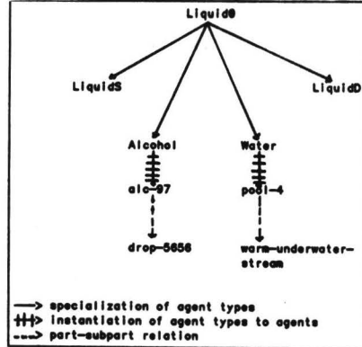
Figure 4-1: Specialization/Instantiation/Parts-Hierarchy
