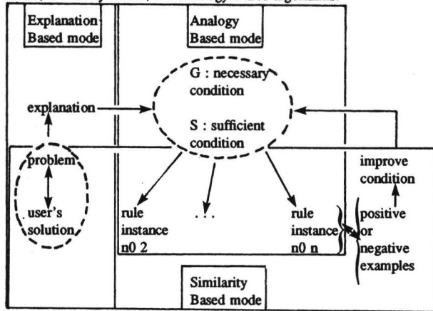
Figure 1. The learning method in DISCIPLE.
