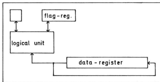
Figure 9: A subprocessor cell of ASSIP-T
