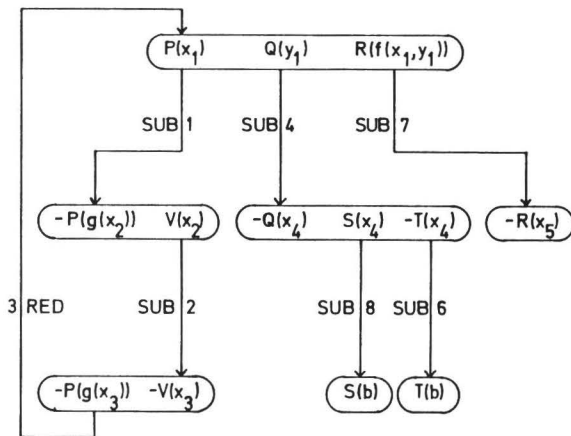
Figure 7: A closed correct deduction plan
