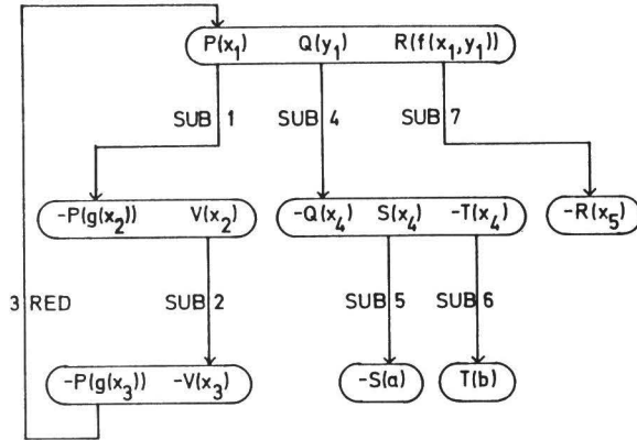
Figure 1: A closed deduction plan
