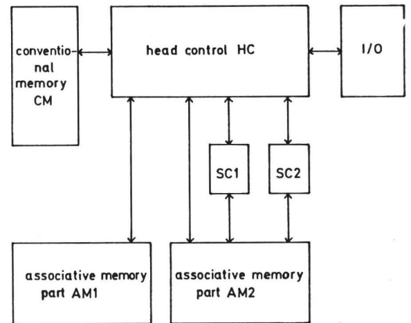
Figure 8: The structure of ASSIP-T
