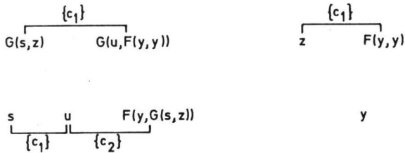
Figure 3: The UwC at the end of the transformation step
