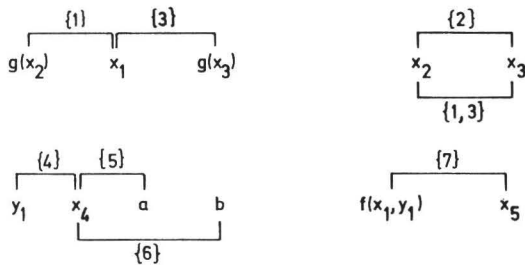
Figure 6: A complete UwC
