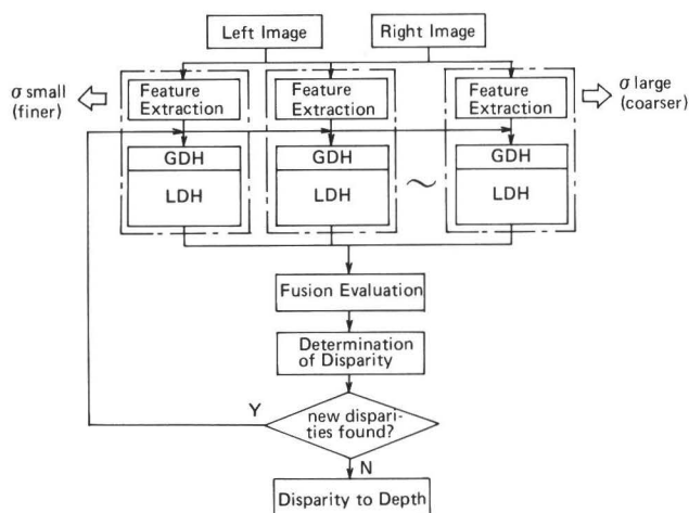
FIGURE 1 BLOCK DIAGRAM OF PARALLEL MATCHING ALGORITHM
