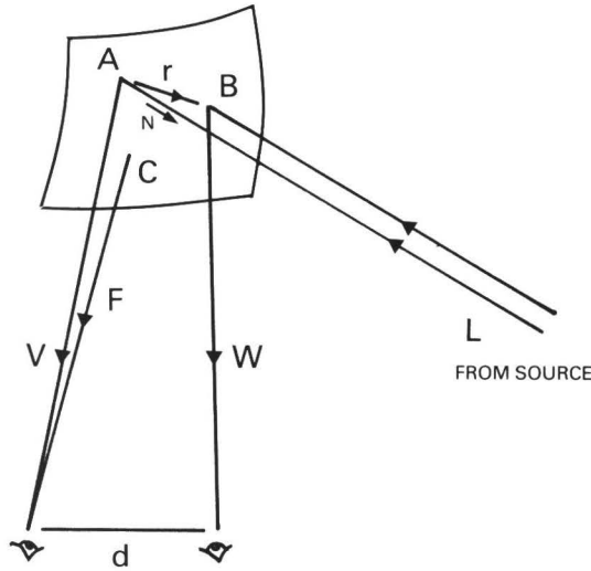
Figure 2: Stereo viewing geometry. Illumination comes from a distant point source, in direction L . Rays to left and right eyes lie along vectors V, W , and strike the surface at points A, B respectively. Surface normals at A, B are N, N' respectively. The vector from A to B is r , and the baseline lies along vector d . A surface feature is assumed to be present nearby, at C , with position vector F relative to the left eye.
