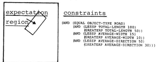
iconic data structure (b)
