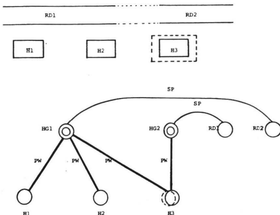
Fig. 15 Suspending unification process
