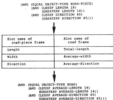
Fig. 10 Attribute translation
