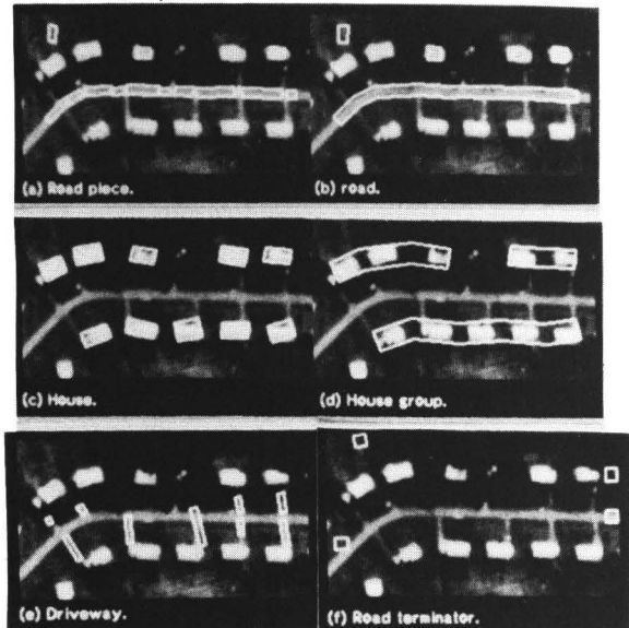
Fig. 16 Final object instances
