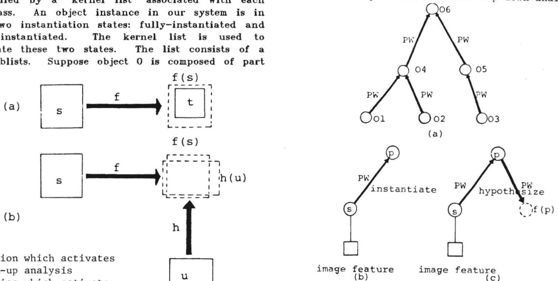
Fig. 5 (a)PW hierarchy (b)Bottom-up instantiation (c)Top-down hypothesis generation
