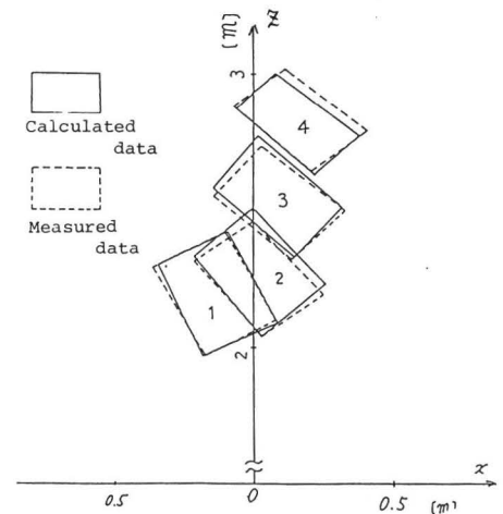
Fig. 6 Results of Experiment compared with Measured Data
