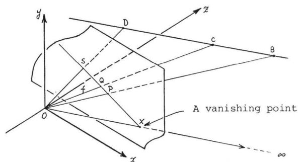
Fig. 3 A Central Projection
