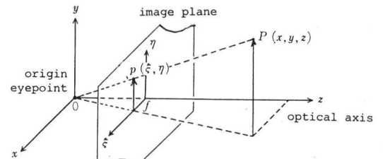
Fig. 1 Coordinates and Central Projection
