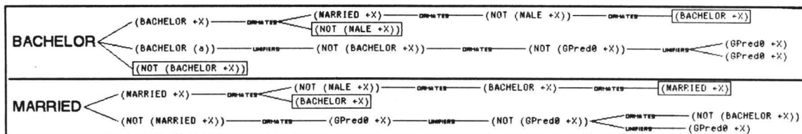
Figure 2. The PCG from BACHELOR and MARRIED
