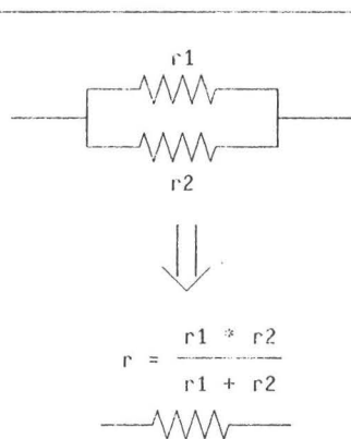
Figure 2: Replacing a pair of parallel resistors by a single resistor.
