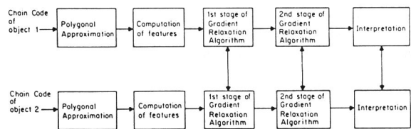
Fig. 1 Block Diagram of the Occlusion Algorithm
