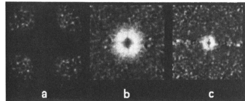
Figure 3: Effect of the Gaussian pyramid levels in the Fourier spectrum. It was obtained by dividing the Fourier spectrum of the original picture by the Fourier spectrum of the filtered picture. a) Elimination of lowest level preserves low frequencies. b) Elimination of the second level attenuates an interior frequency band. c) Elimination of the third level attenuates smaller interior frequencies.
