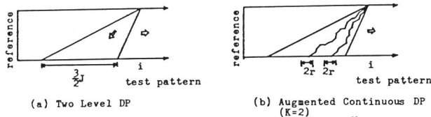
Fig.5 Range of m for the calculation of D^n(m+1:i)
