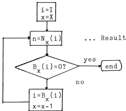
Fig.2 Decision process of recognition result (known length of string)
