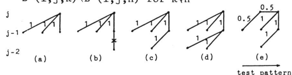
Fig.4 Asymmetric DP pass and weight
