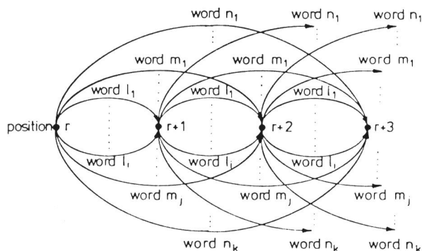
figure 3: word hypotheses
