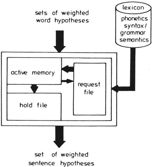
figure 4: intelligence stage
