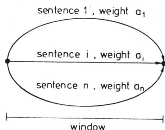
figure 5: sentence hypotheses
