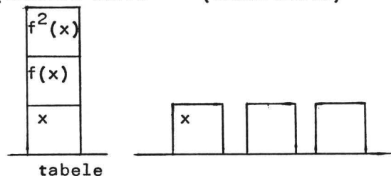
Fig. 1 Clearing a block x ; f(x) =_{\text{Df}} \cup(ON(u, x)) ( \cup : jota operator)
